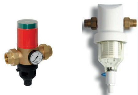
Backflow preventer
